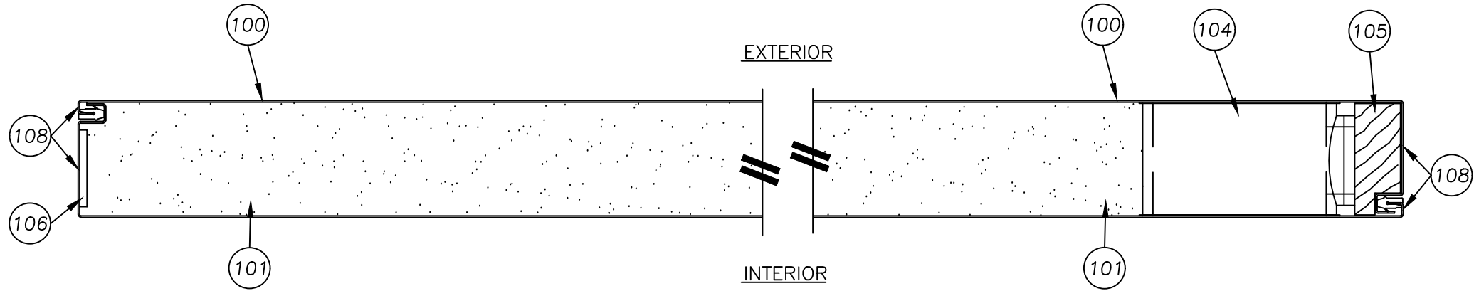
2 HORIZONTAL CROSS SECTION 4 MASONITE STEEL OPAQUE DOOR
